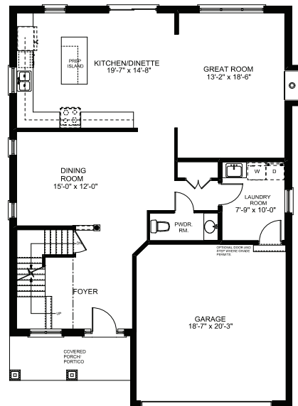
GROUND FLOOR PLAN - 1246 sf
