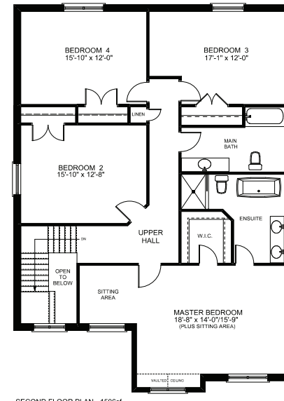
SECOND FLOOR PLAN - 1506sf ELEVATION A
